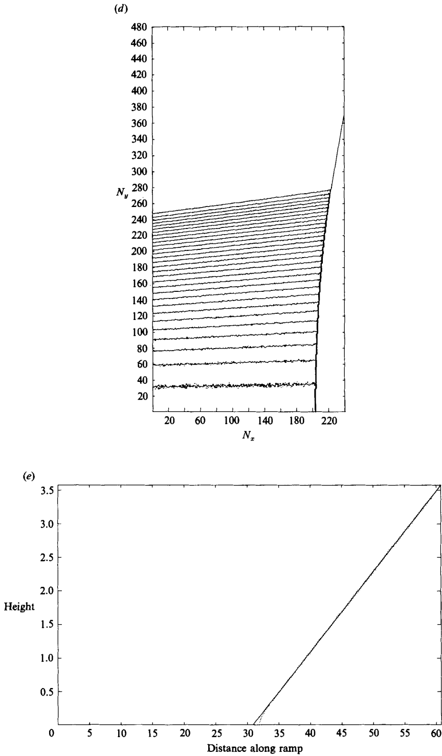
FIGURE 7. Finite difference calculations for the contours of a von Neumann reflection for which his theory has no acceptable Mach reflection solutions for argon. \gamma = \frac{5}{3} , \xi_t = 0.889737 , M_t = 1.0483 , \theta = 10^\circ . For other information see the caption to figure 5.
