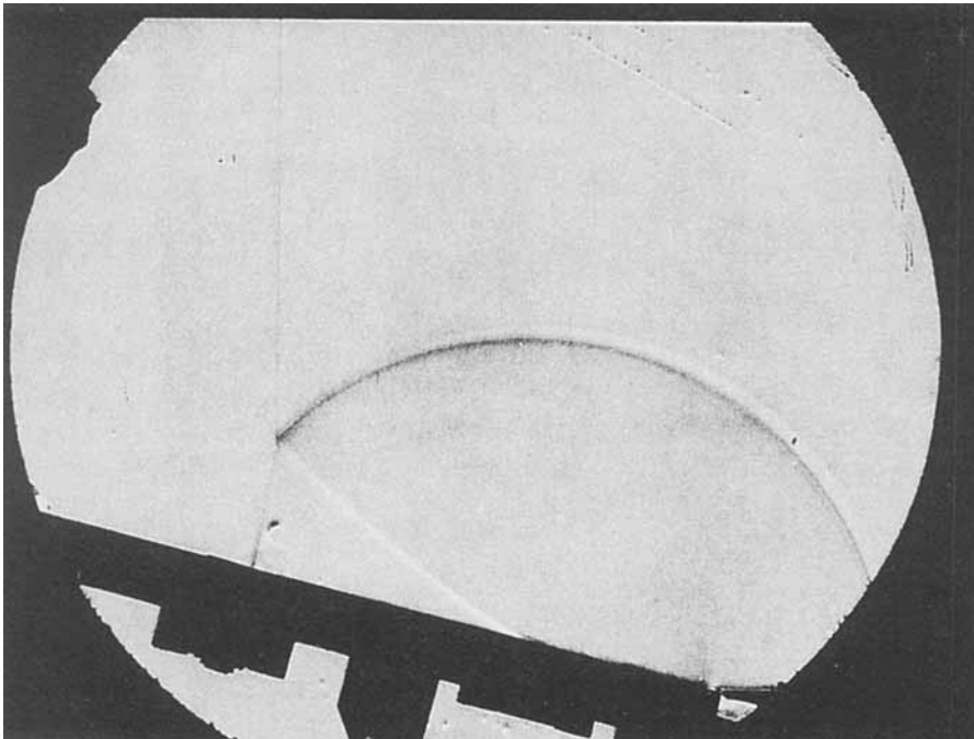
FIGURE 9. Schlieren photograph of a von Neumann reflection over a concave corner model in argon for run number 81. In this case the theory of weak MR requires that \beta_1 > \frac{1}{2}\pi . \gamma = \frac{5}{3} , \xi_i = 0.403 , M_i = 1.48 , \theta = 14.58^\circ .
