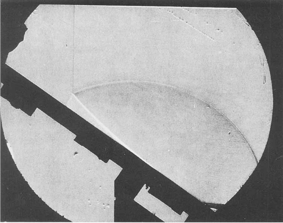
FIGURE 8. Schlieren photograph of a weak Mach reflection over a concave corner model in argon for run number 85. \gamma = \frac{5}{3} , \xi_i = 0.409 , M_i = 1.47 , \theta = 34.60^\circ .
