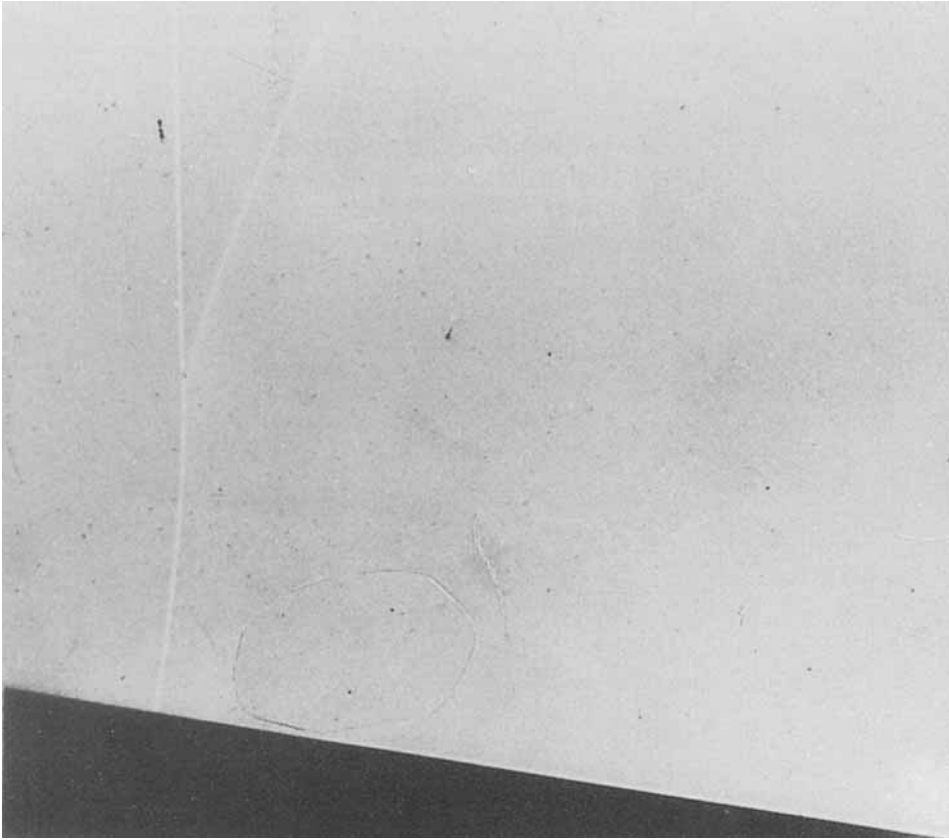
FIGURE 10. Schlieren photograph of a von Neumann reflection over a concave model in argon for which Mach reflection has no physically acceptable solutions. \gamma = \frac{5}{3} , \xi_t = 0.889 , M_i = 1.05 , \theta = 10^\circ .
