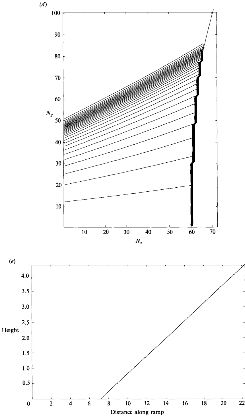
FIGURE 6. Finite difference calculations for the contours for the conditions of the von Neumann reflection with run number 81 in argon. \gamma = \frac{5}{3} , \xi_i = 0.403 , M_1 = 1.48 , \theta = 14.58^\circ . For these conditions the weak Mach reflection theory requires that \beta_1 > \frac{1}{2}\pi . For other information see the caption to figure 5.
